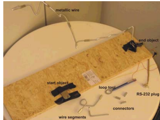
figure 1: First prototype of the HotWire.
